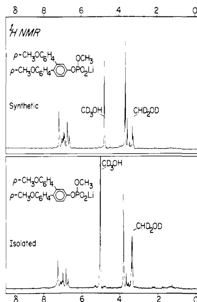
Figure 1. 1 H NMR spectra of synthetic lithium methyl 3,4-dianisylphenyl phosphosphate and of the product of the rearrangement of 4,4-dianisylcyclohexadienone induced by methyl metaphosphate.
